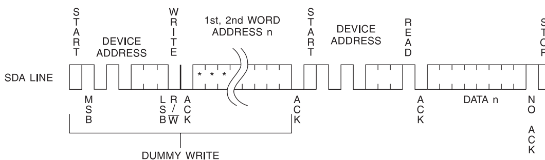
Figure 12-5. Random Read
